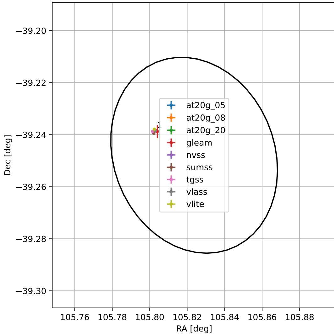
4FGL J0703.2-3914
