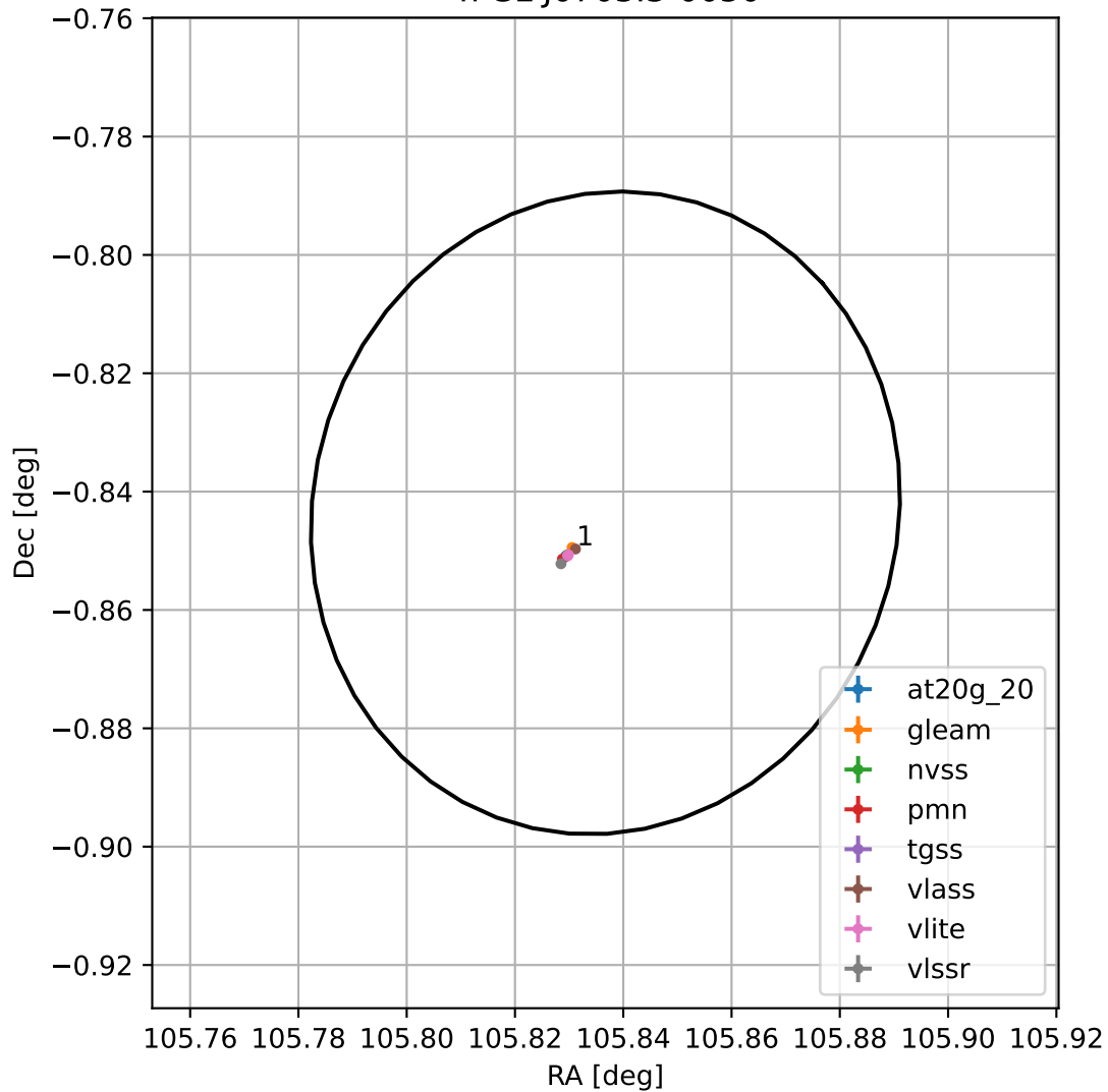
4FGL J0703.3-0050
