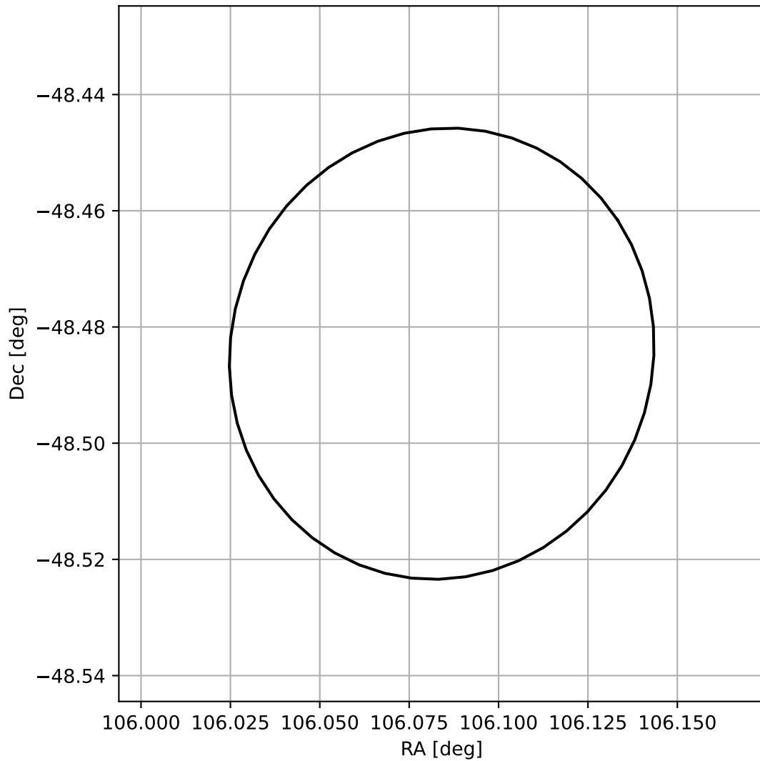
4FGL J0704.3-4829
