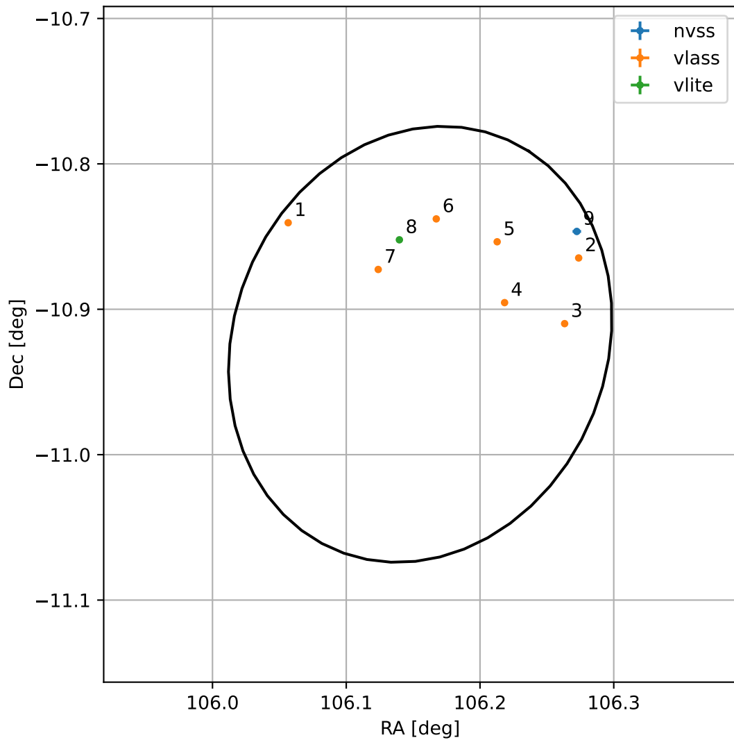
4FGL J0704.6-1055
