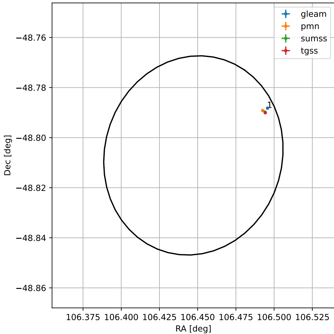
4FGL J0705.7-4848
