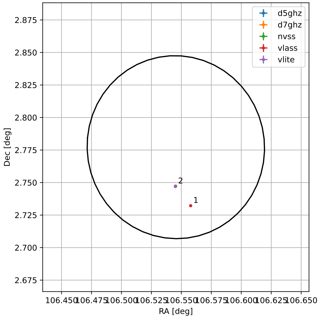
4FGL J0706.1+0246
