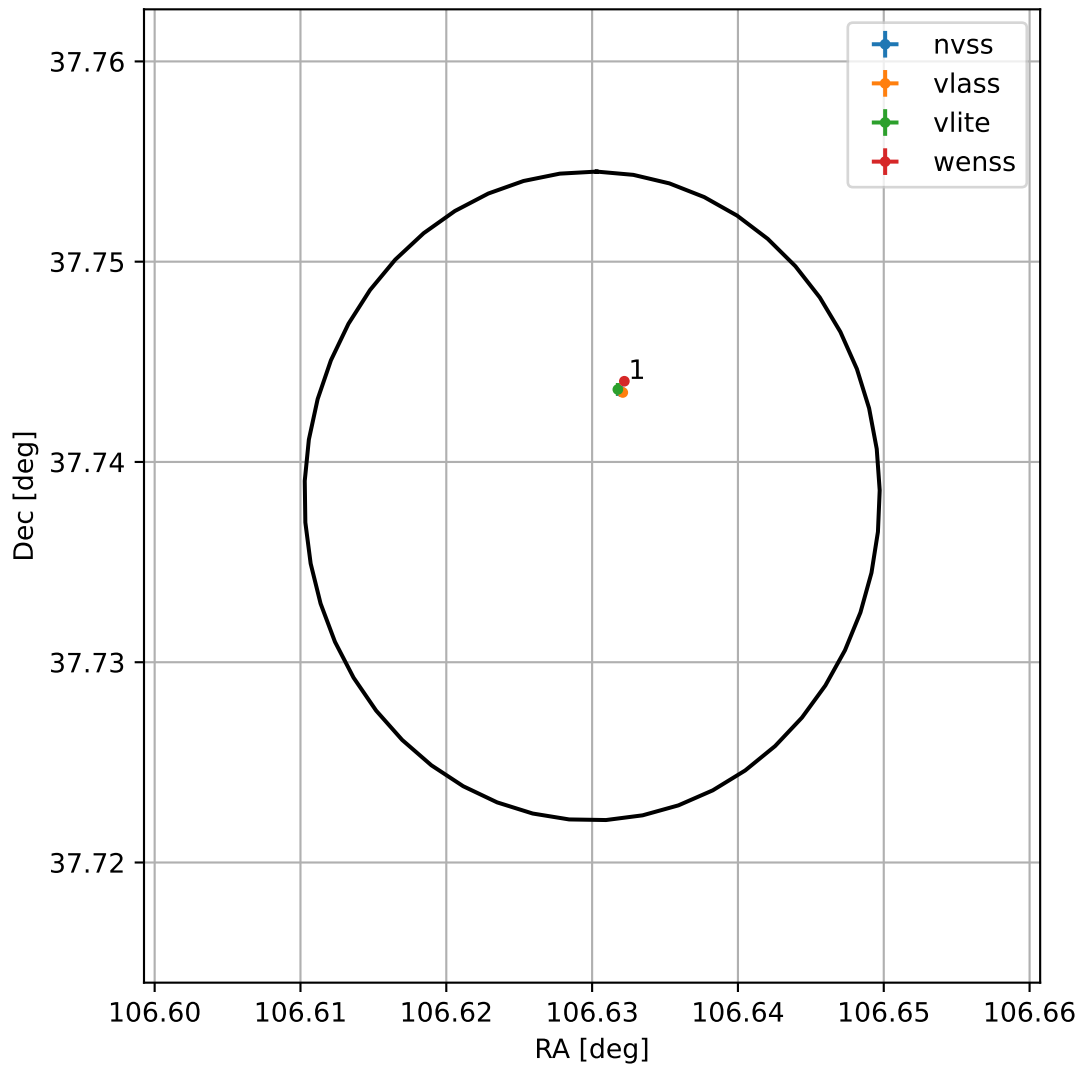
4FGL J0706.5+3744
