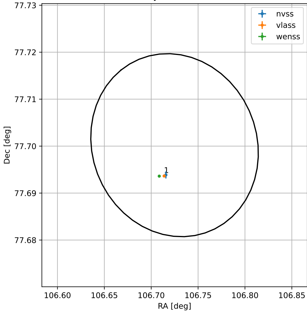
4FGL J0706.8+7742
