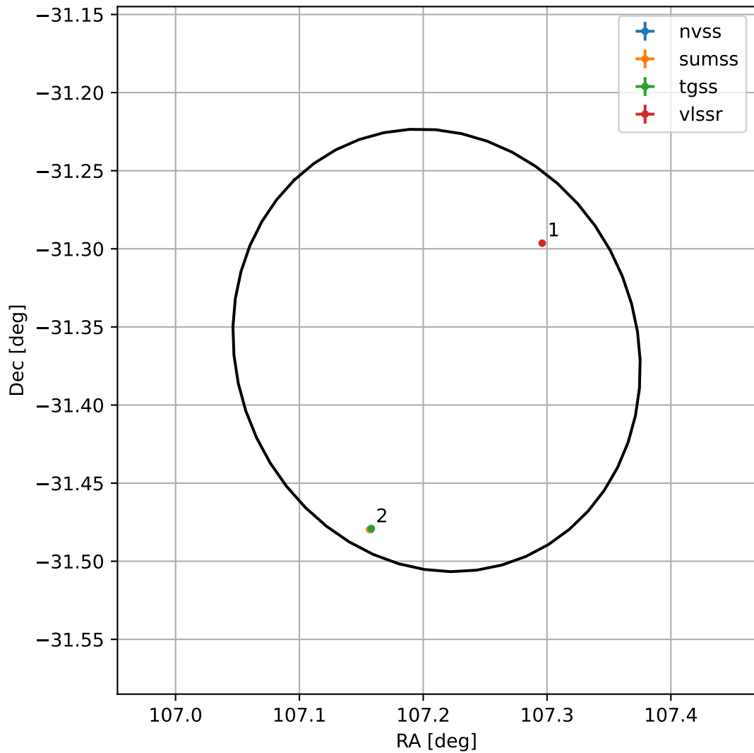
4FGL J0708.8-3121
