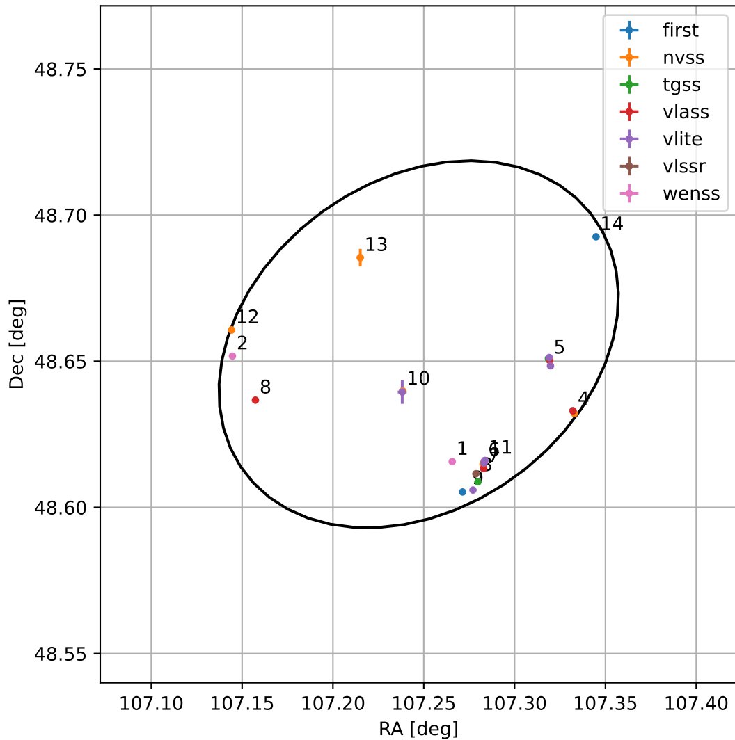
4FGL J0708.9+4839
