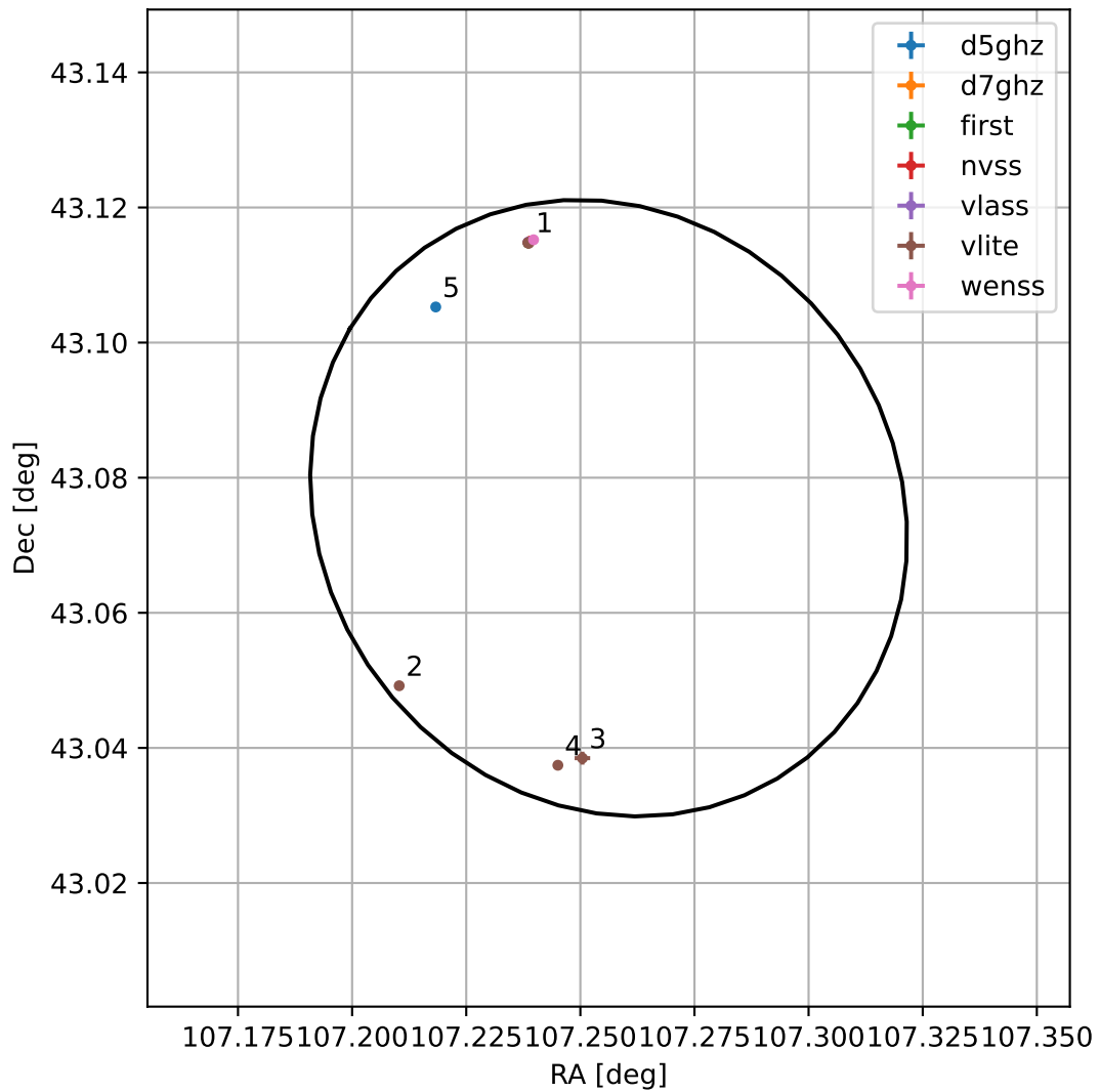
4FGL J0709.0+4304
