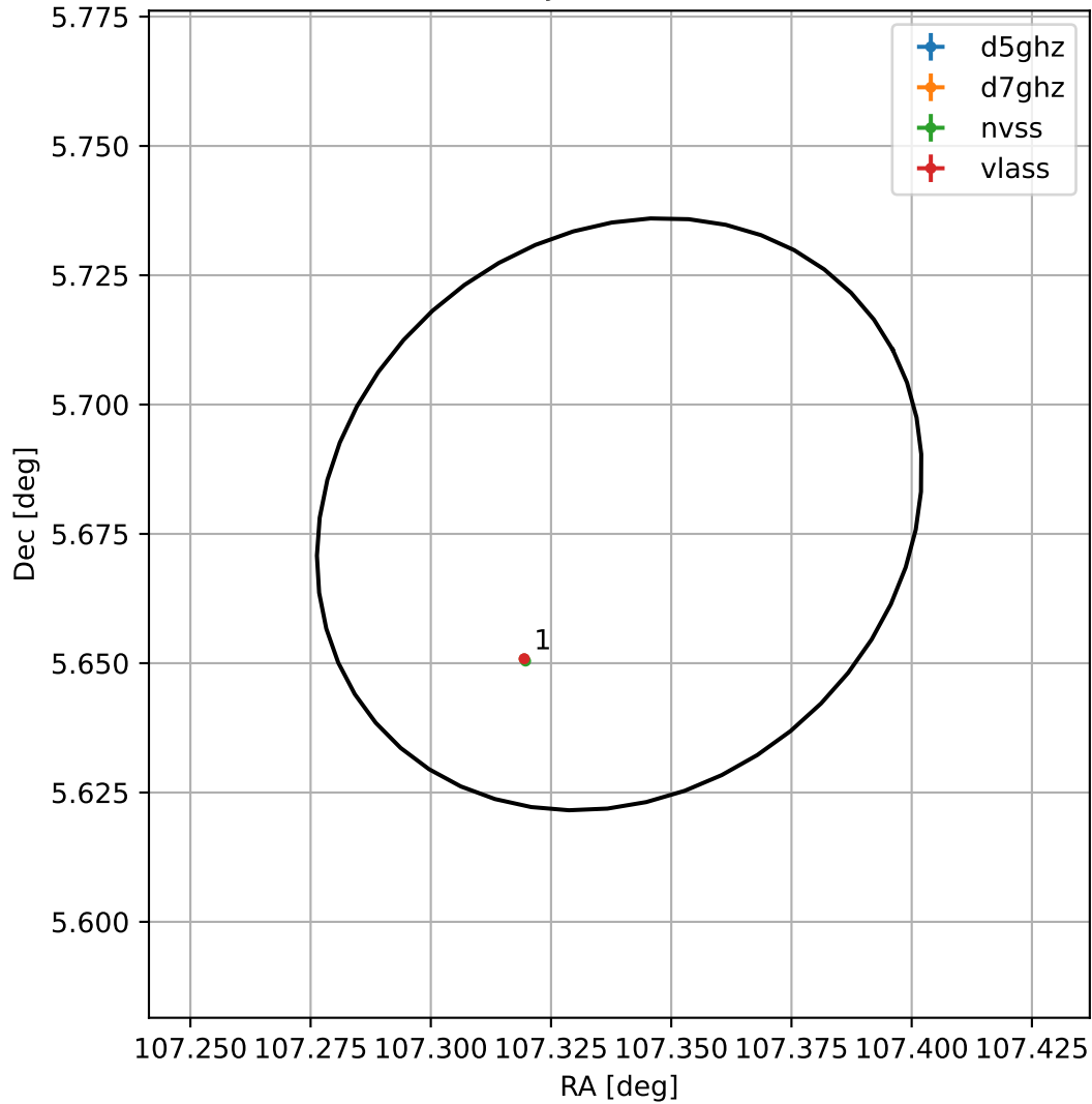
4FGL J0709.3+0540
