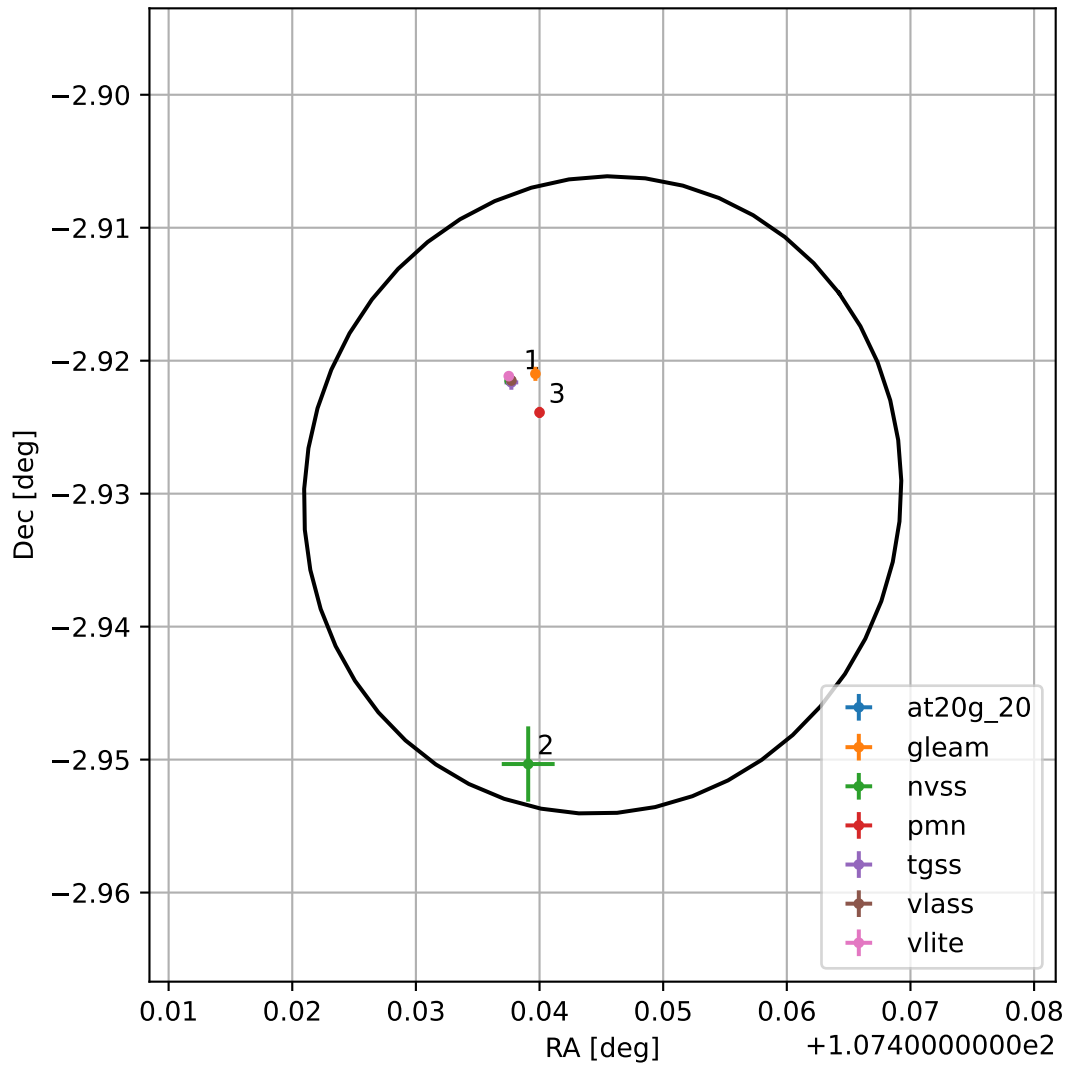
4FGL J0709.7-0255
