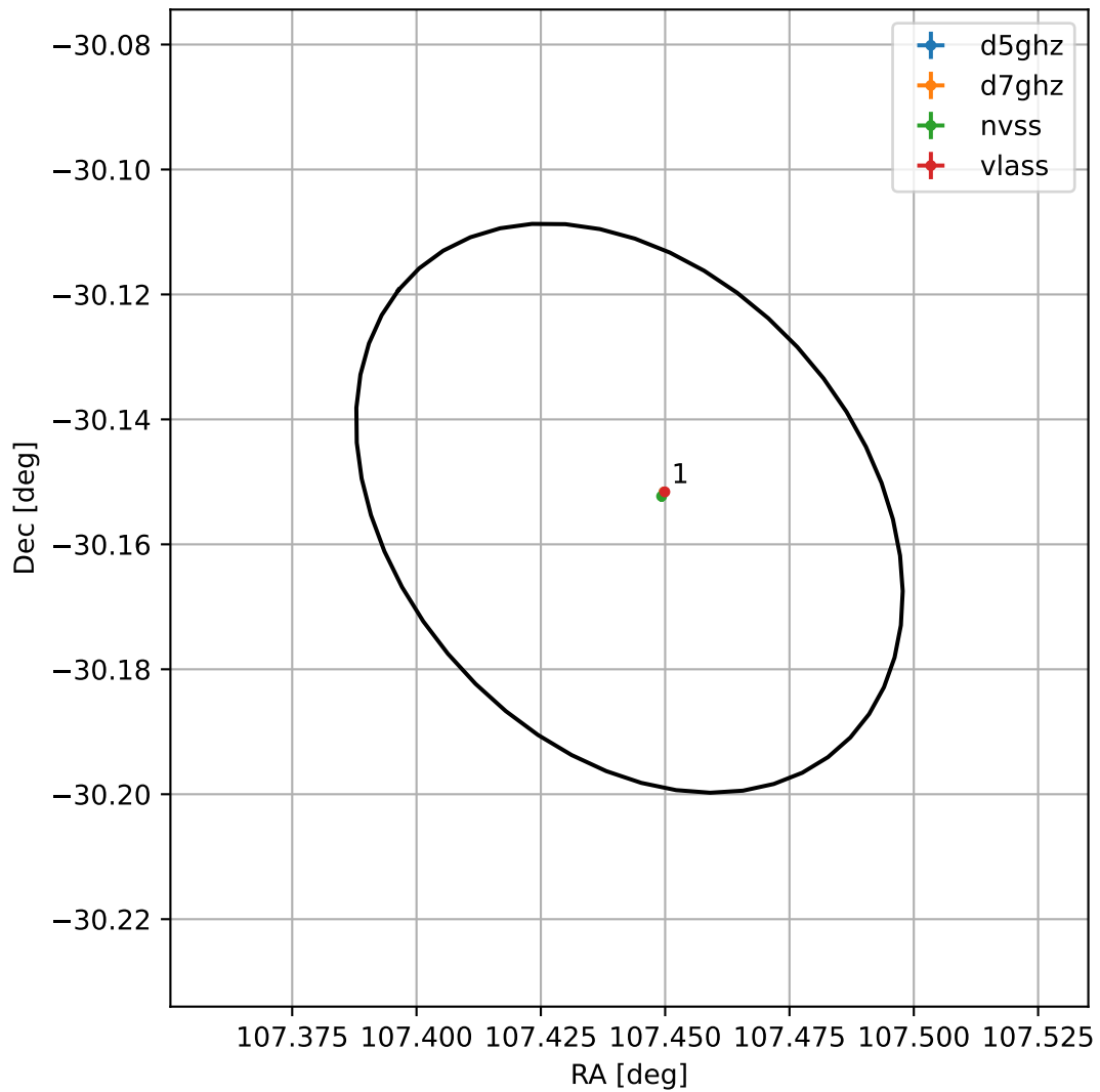
4FGL J0709.7-3009
