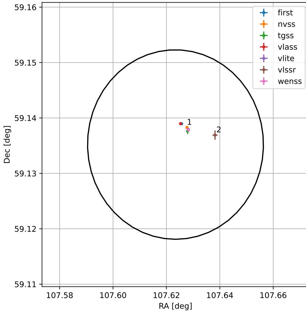
4FGL J0710.4+5908
