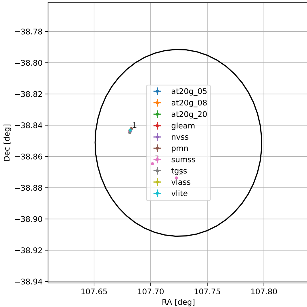
4FGL J0710.8-3851
