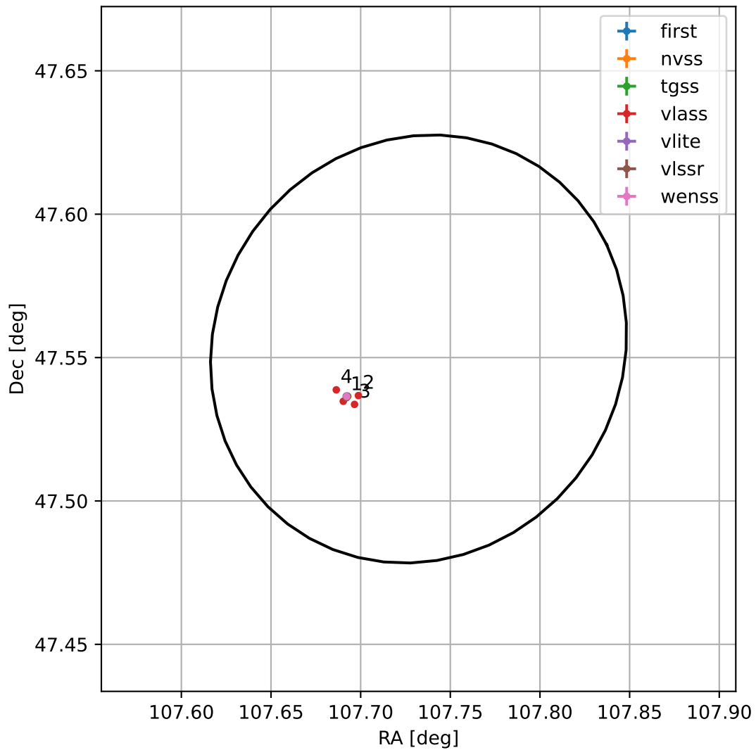
4FGL J0710.9+4733
