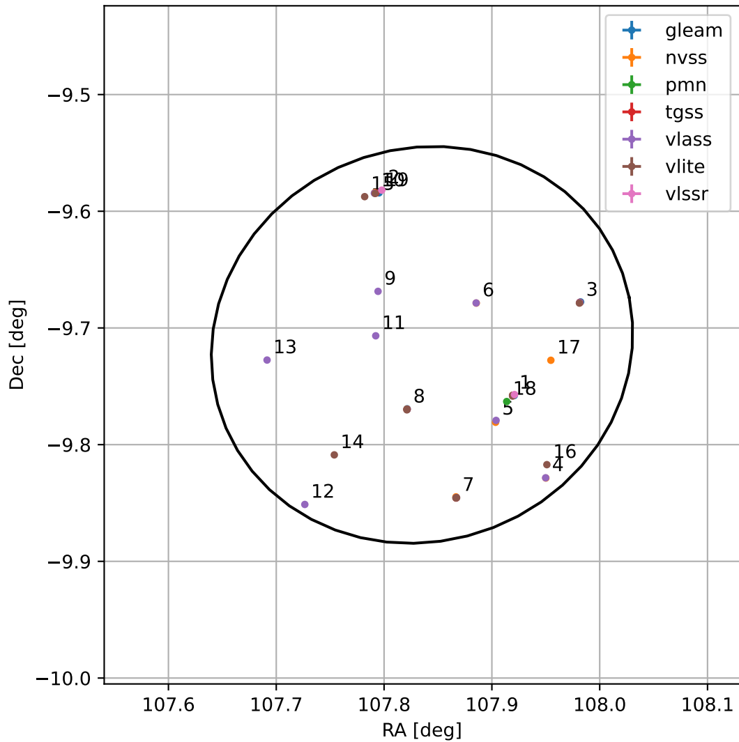
4FGL J0711.3-0942
