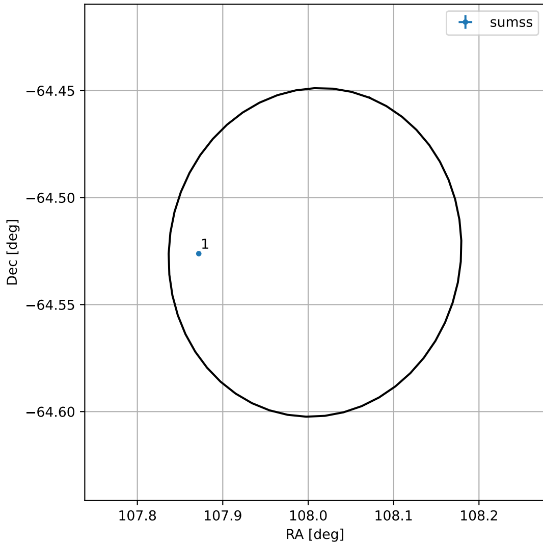
4FGL J0712.0-6431
