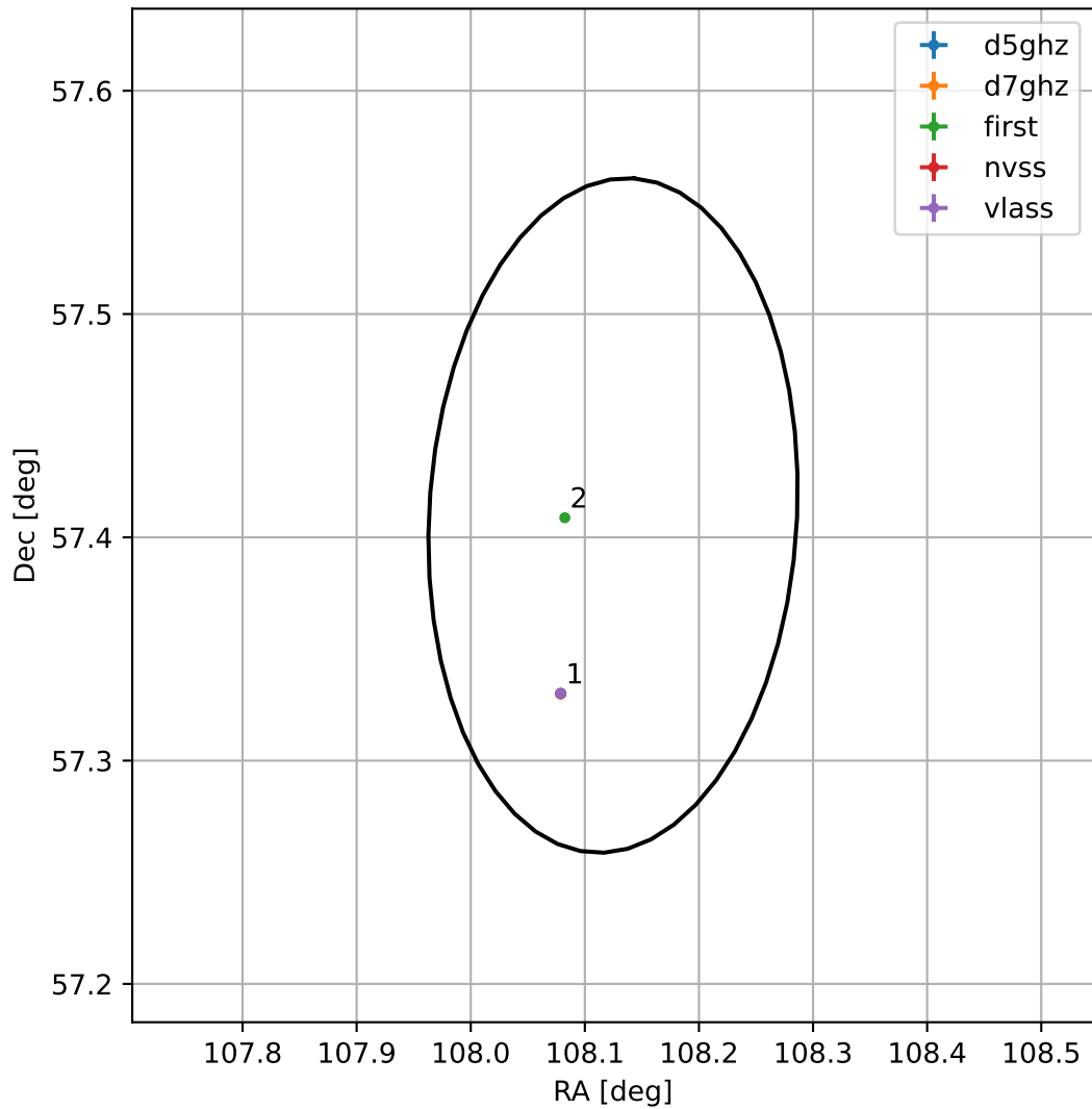
4FGL J0712.4+5724
