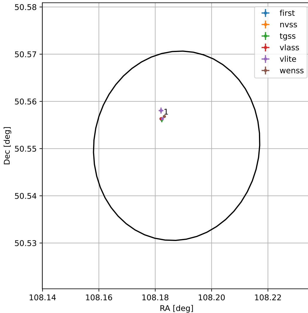
4FGL J0712.7+5033
