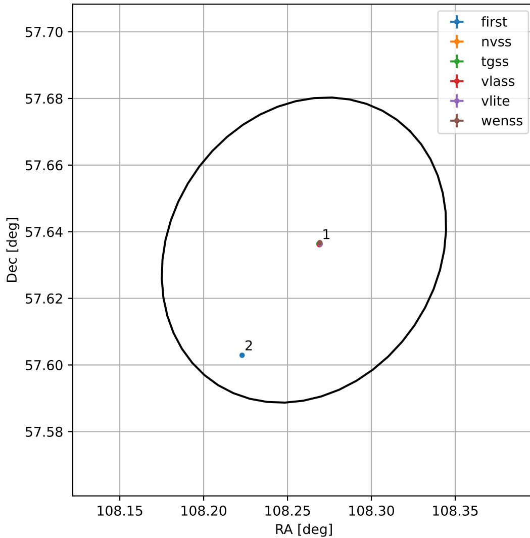
4FGL J0713.0+5738
