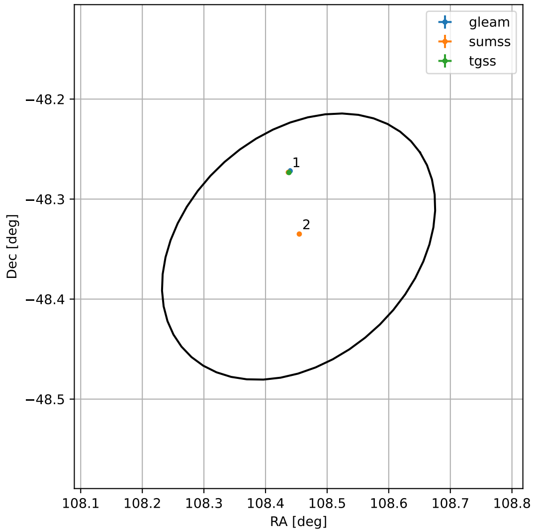
4FGL J0713.8-4820
