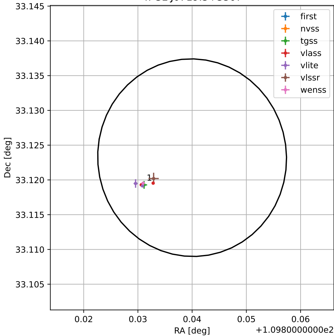
4FGL J0719.3+3307
