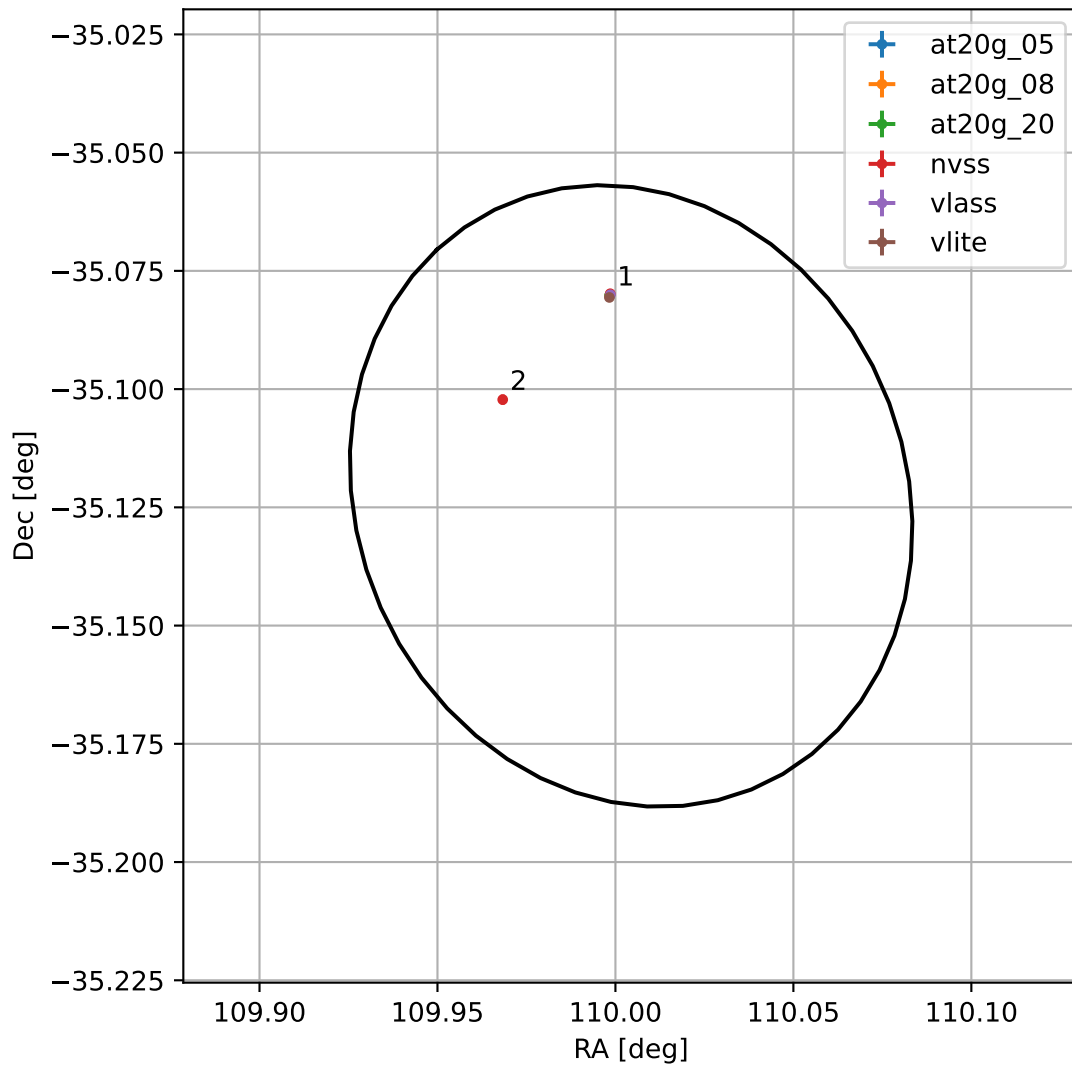
4FGL J0720.0-3507
