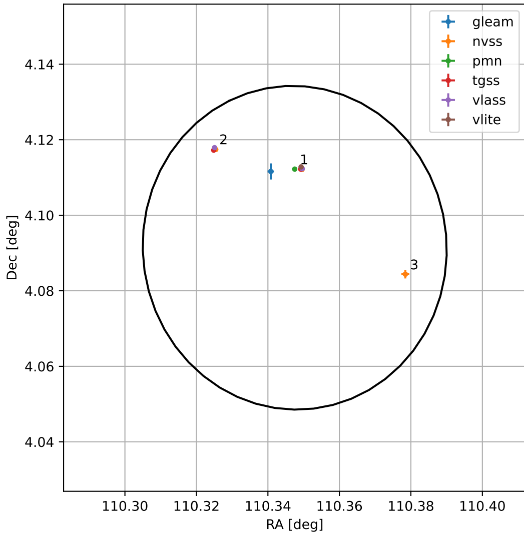
4FGL J0721.3+0405
