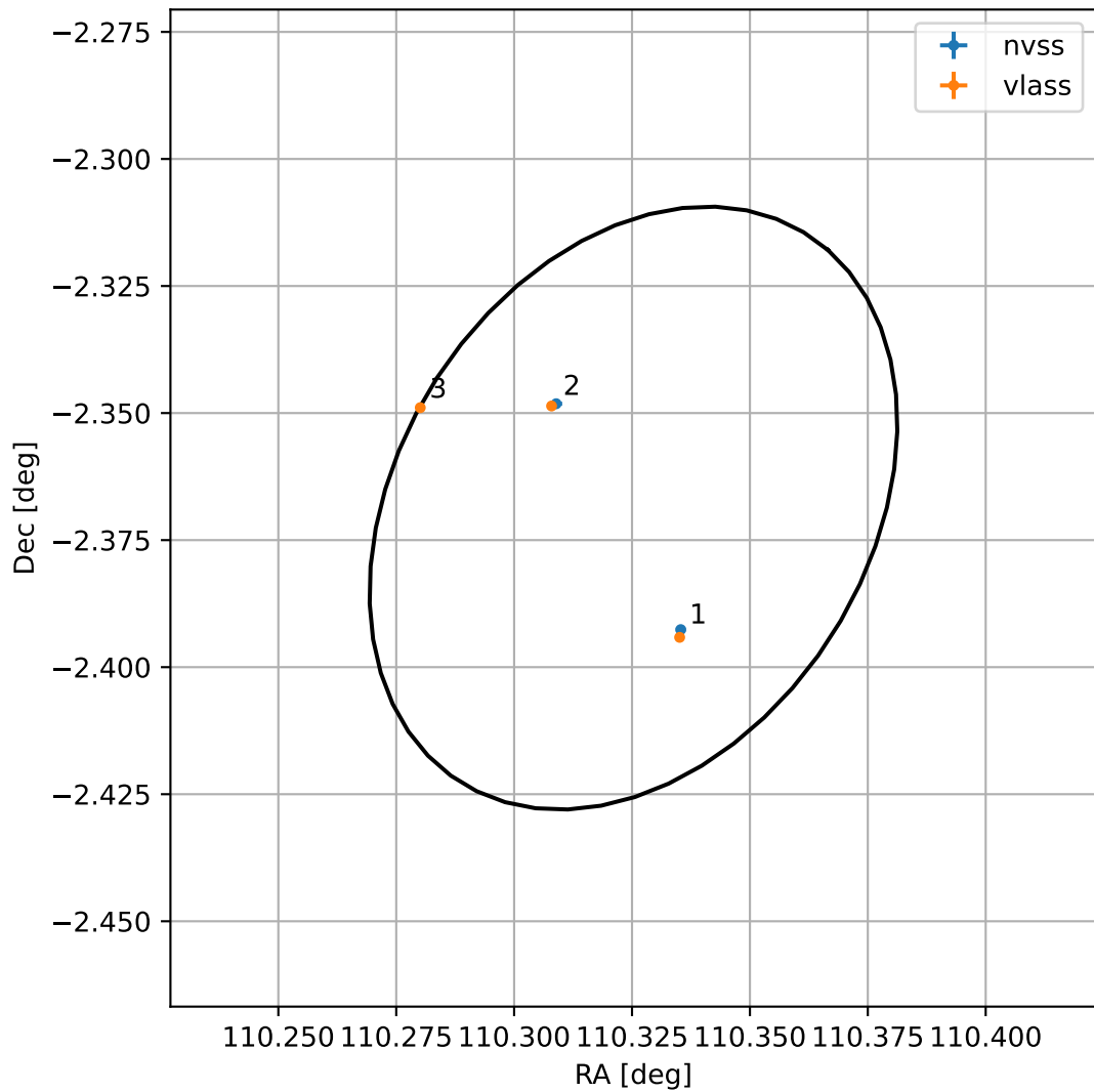
4FGL J0721.3-0222
