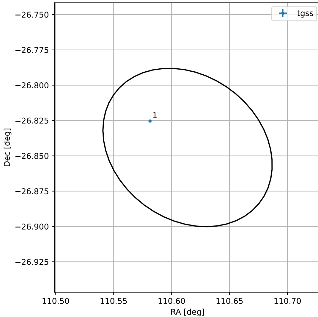
4FGL J0722.4-2650
