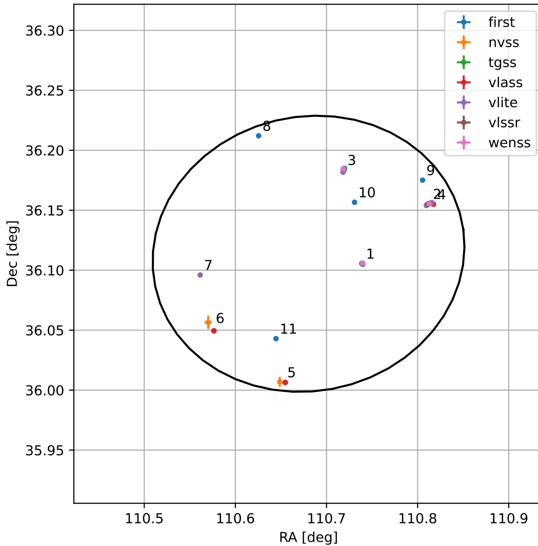
4FGL J0722.7+3606
