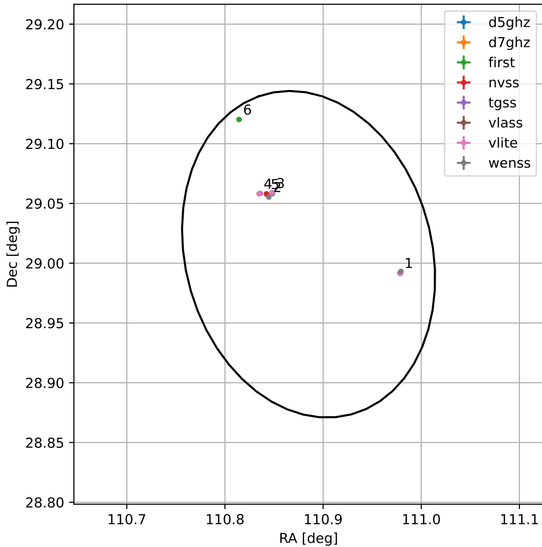
4FGL J0723.5+2900
