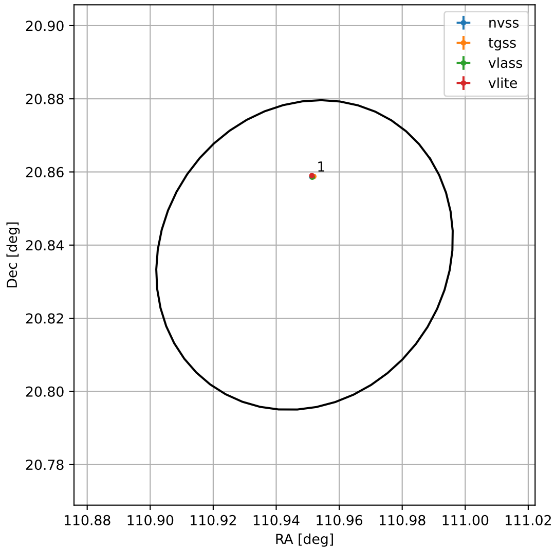
4FGL J0723.7+2050
