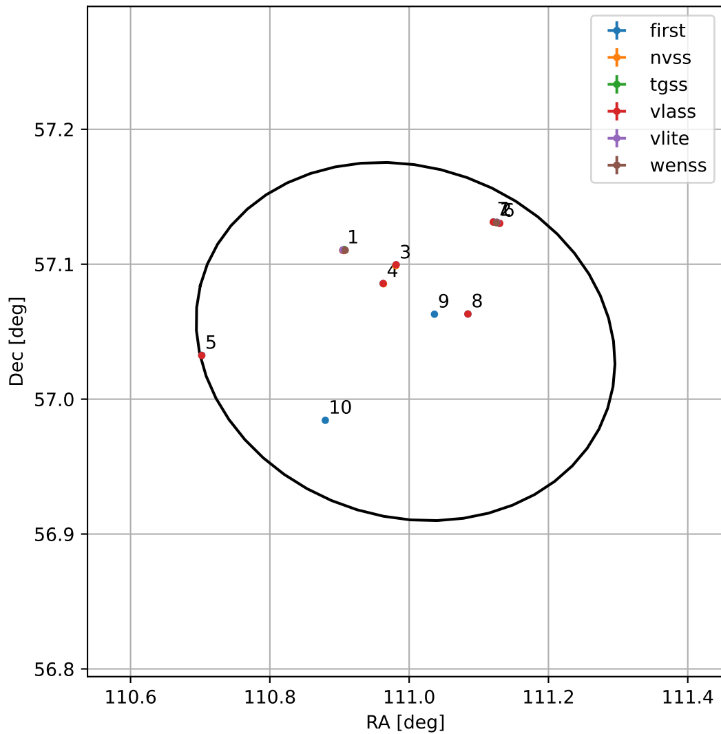
4FGL J0723.9+5702
