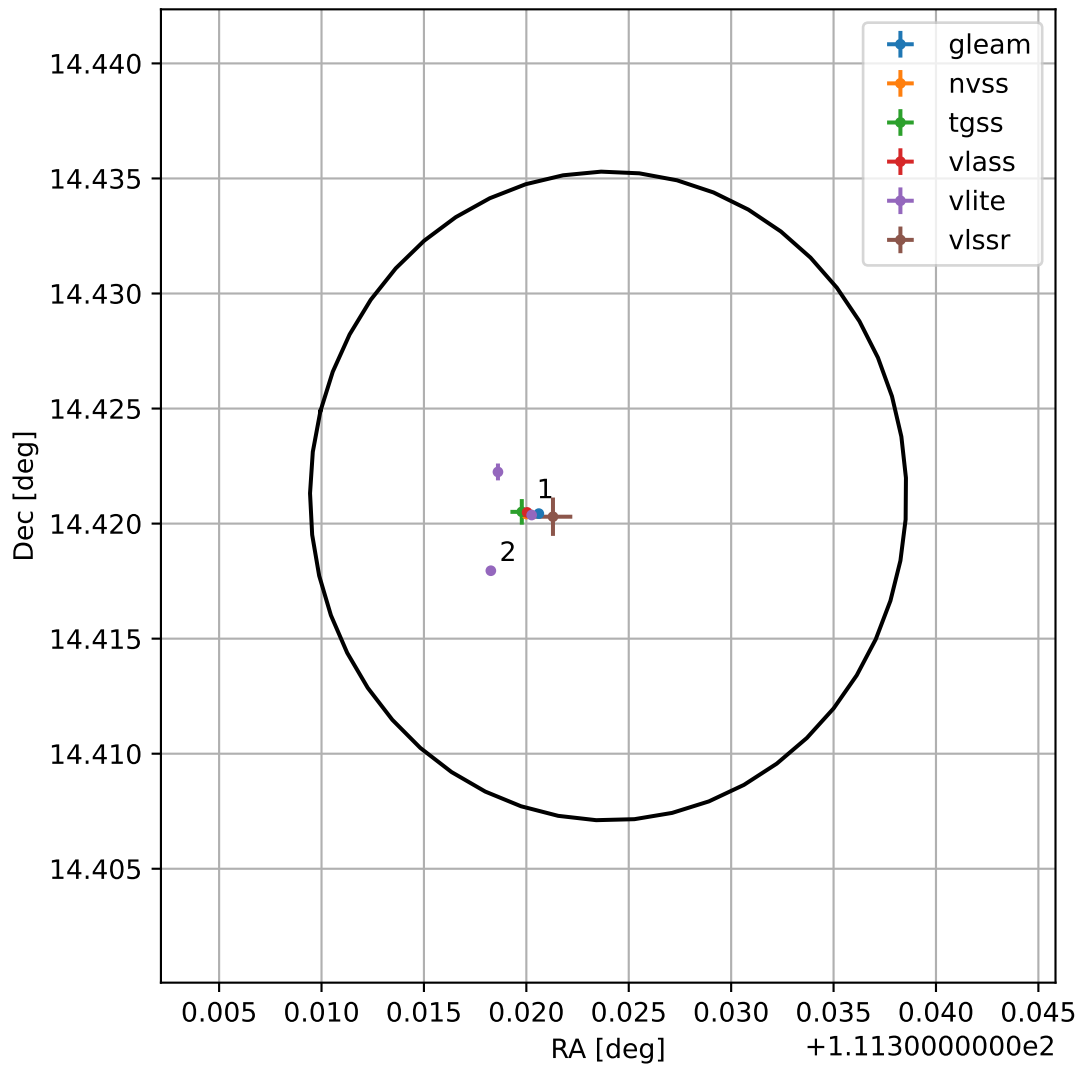
4FGL J0725.2+1425
