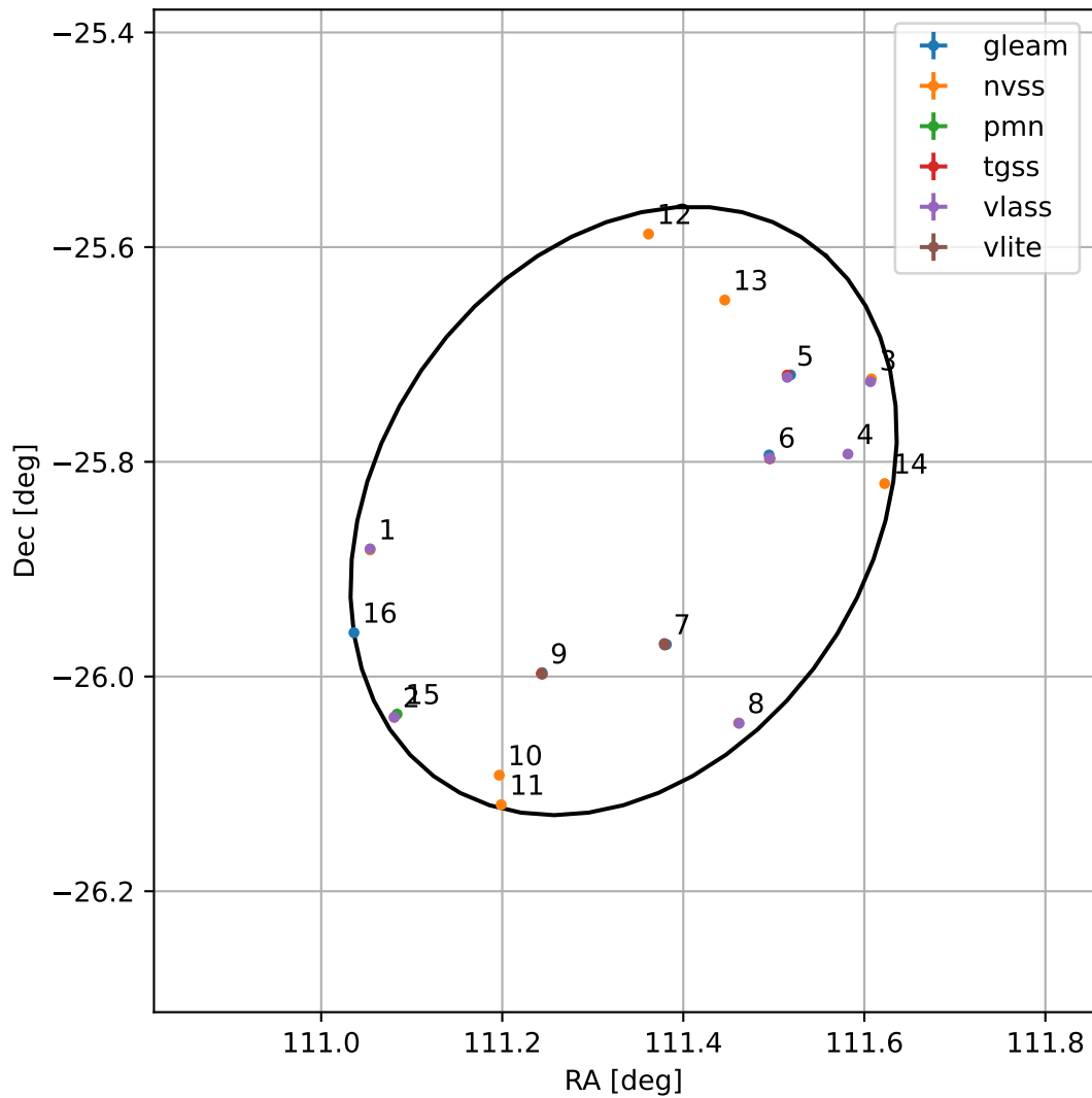
4FGL J0725.3-2550
