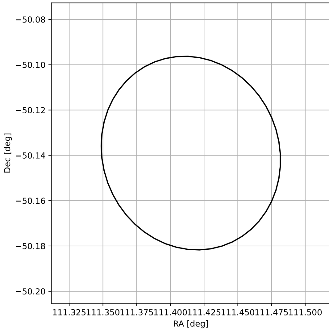
4FGL J0725.6-5008
