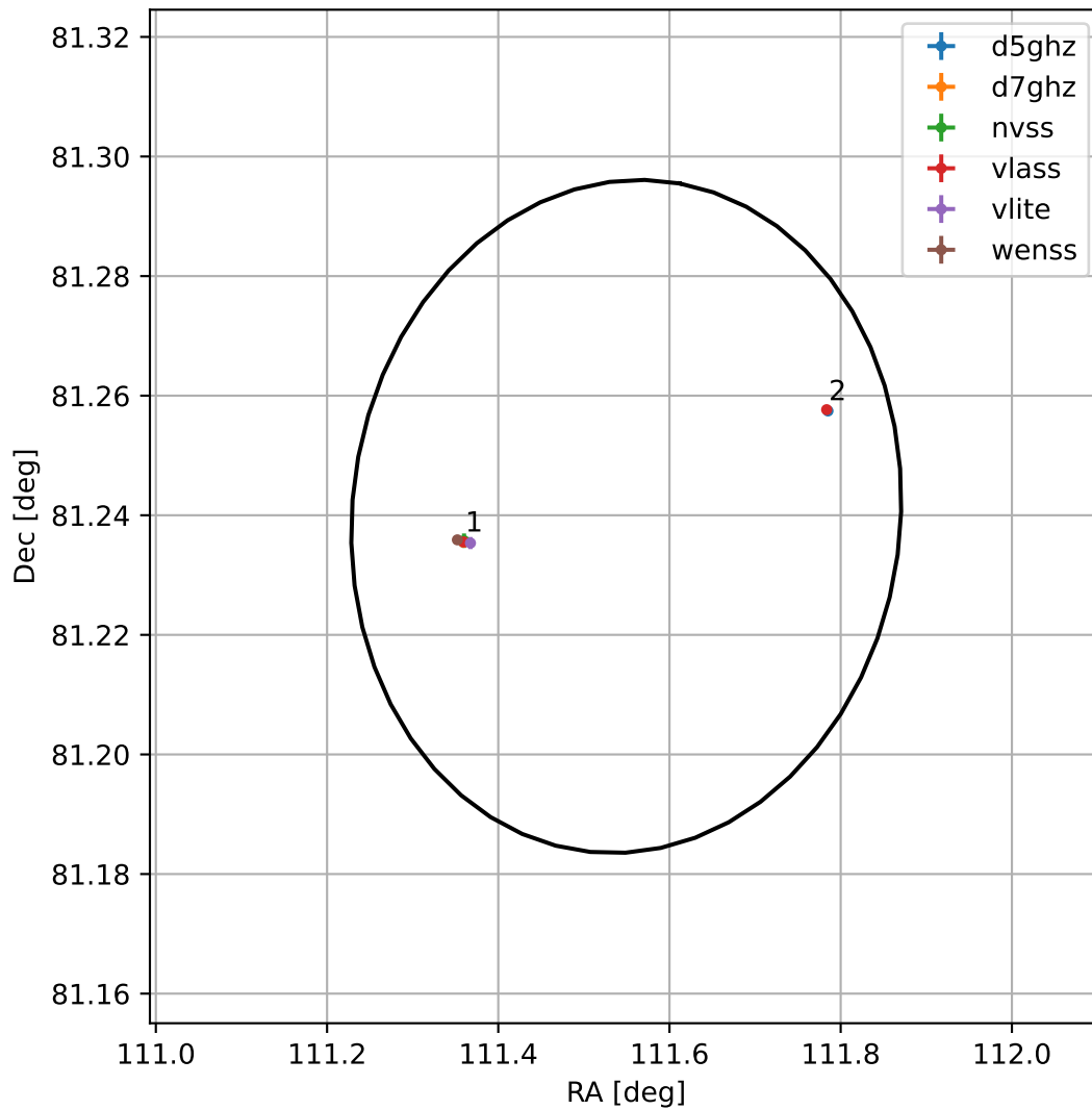
4FGL J0726.1+8114
