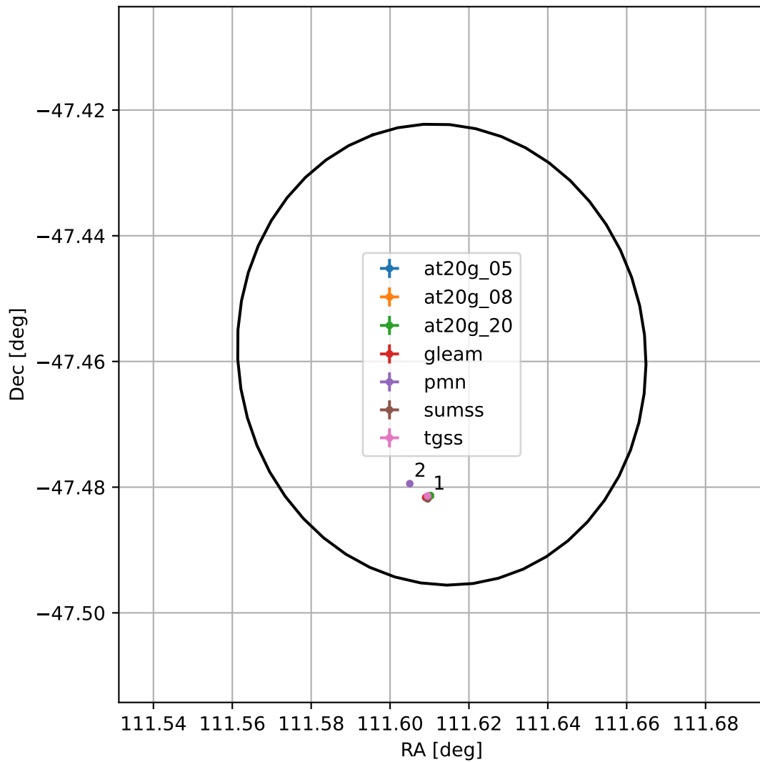
4FGL J0726.4-4727
