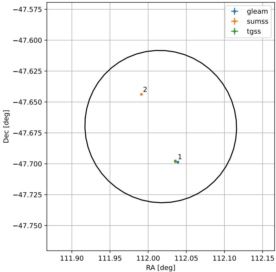
4FGL J0728.0-4740
