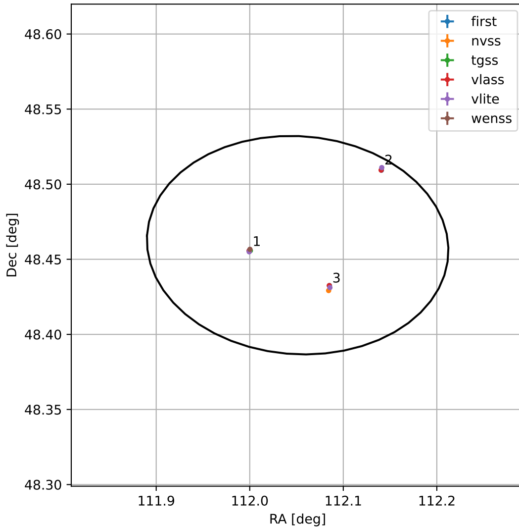
4FGL J0728.2+4827
