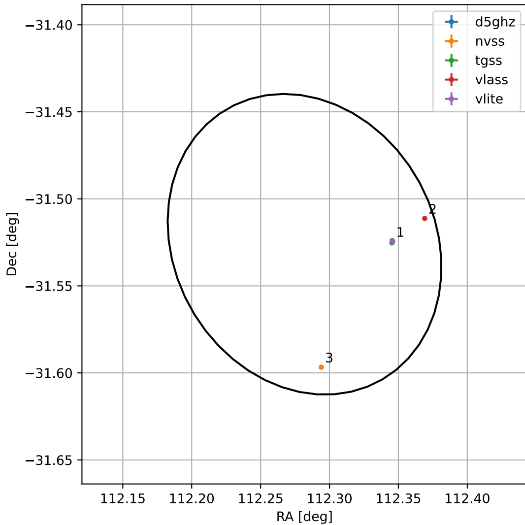
4FGL J0729.1-3131
