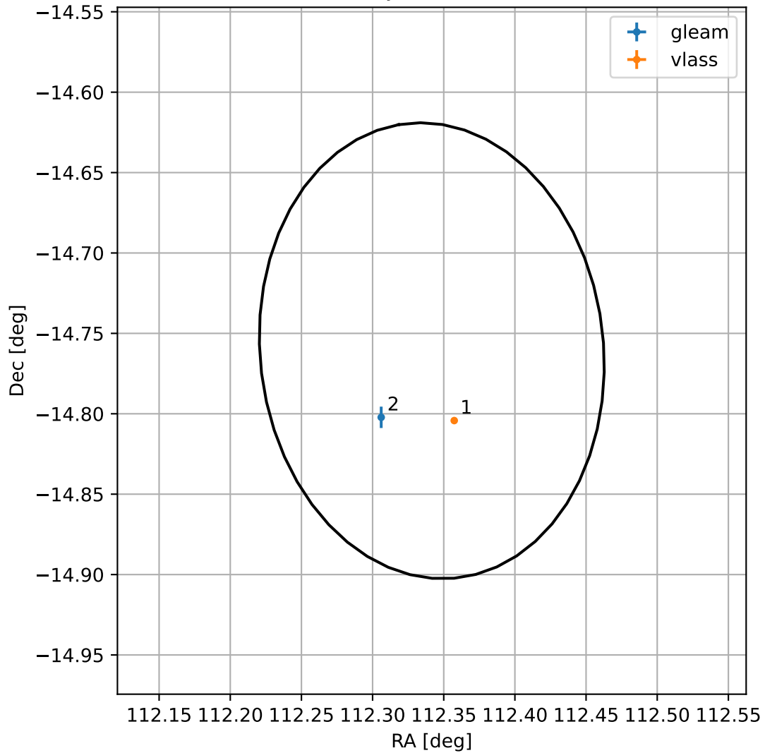
4FGL J0729.3-1445
