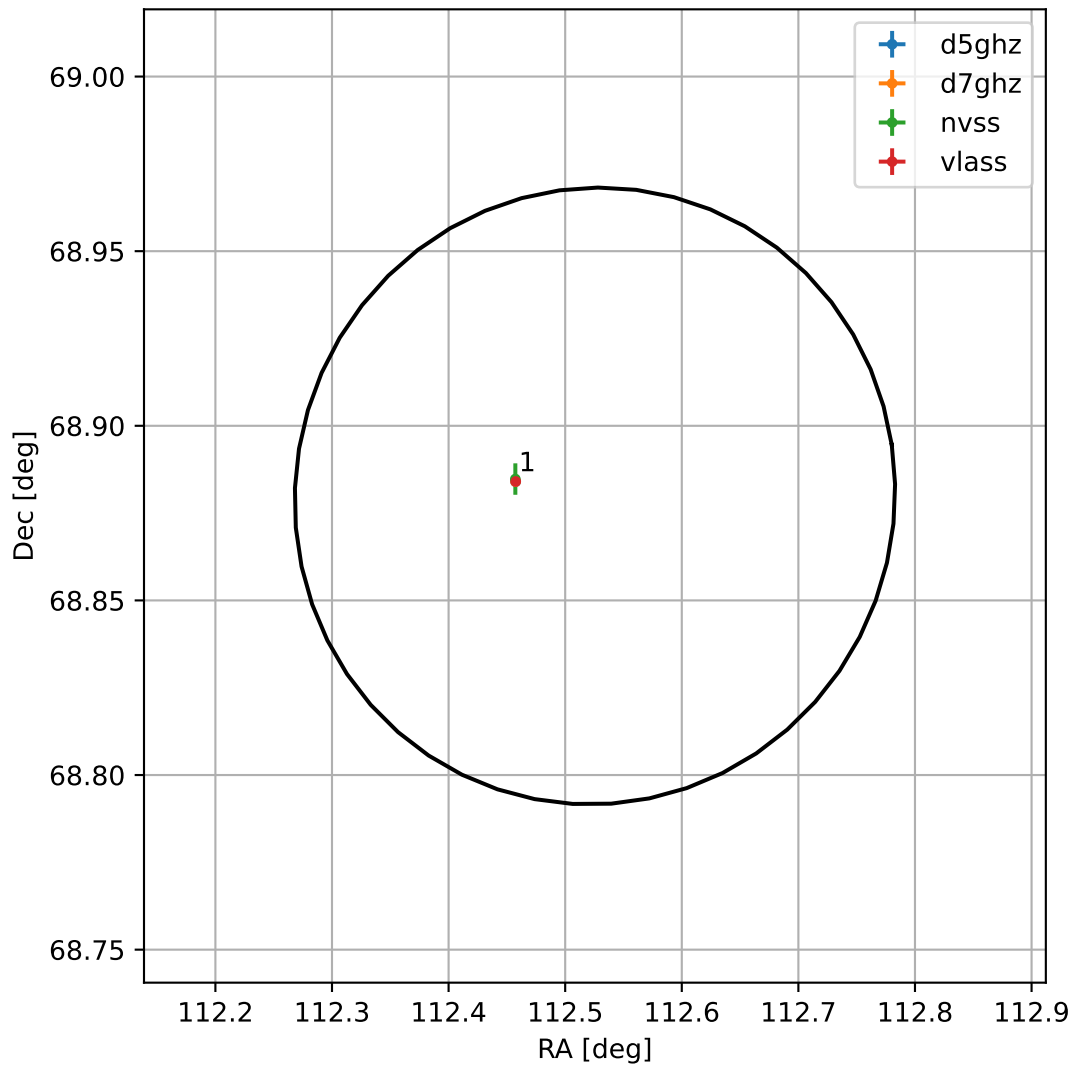
4FGL J0730.1+6852
