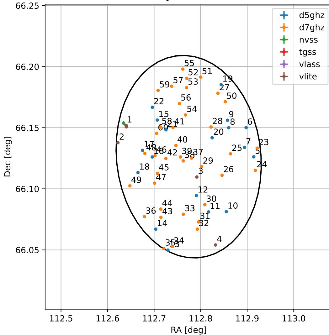
4FGL J0731.0+6607
