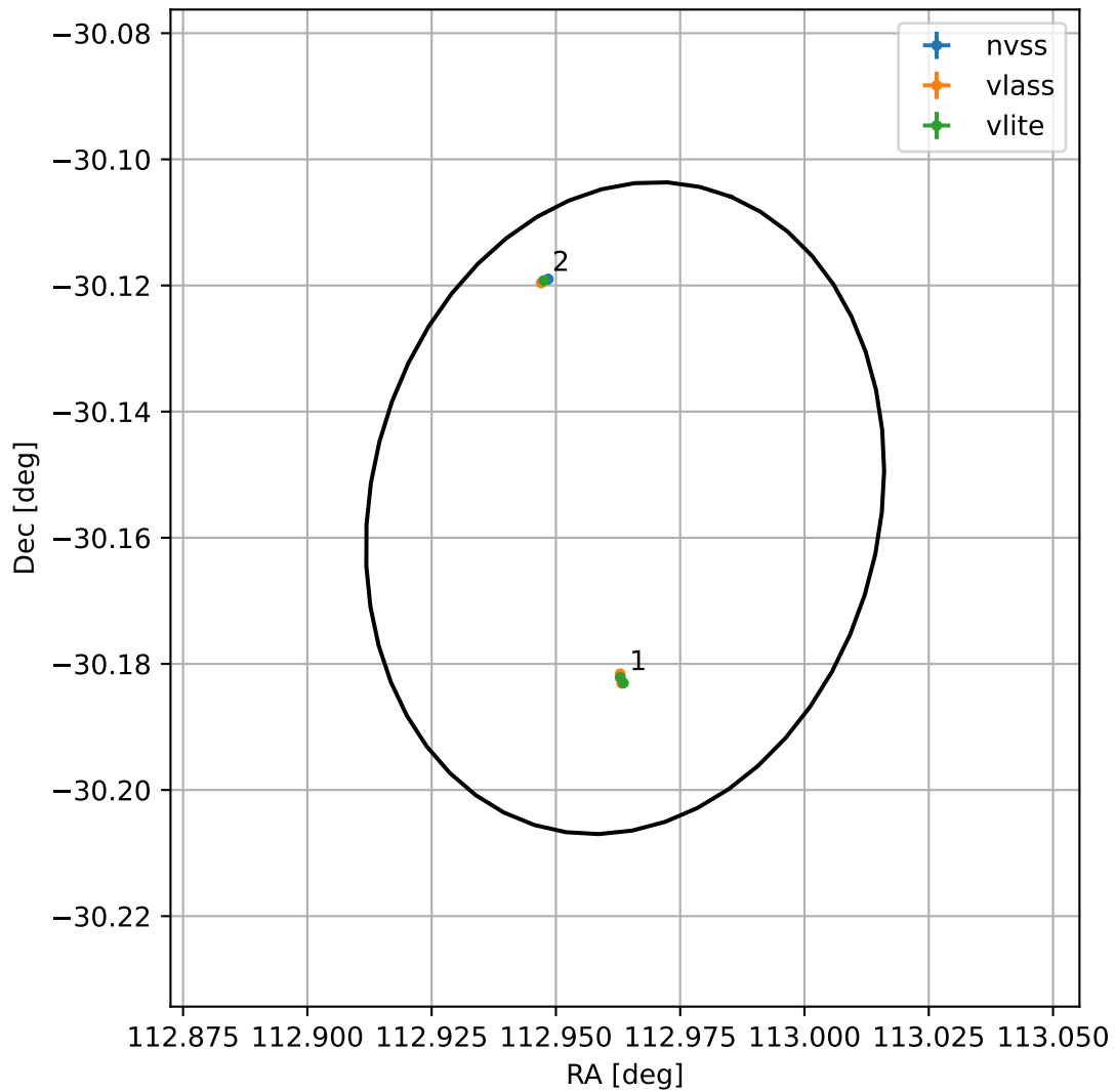
4FGL J0731.8-3009
