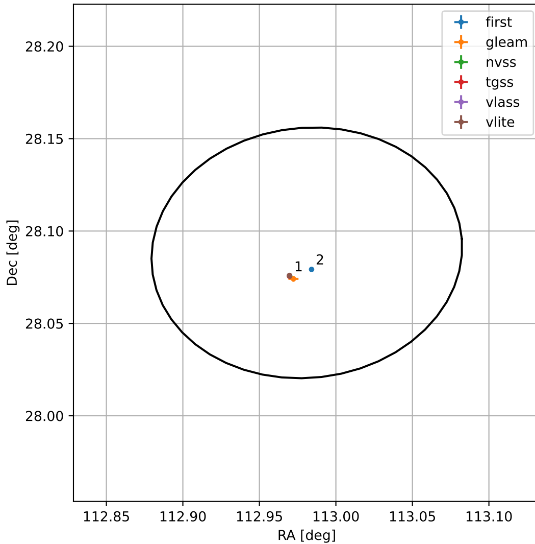
4FGL J0731.9+2805
