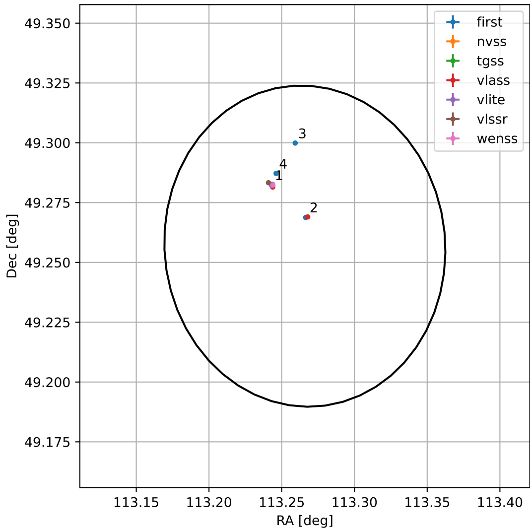
4FGL J0733.0+4915
