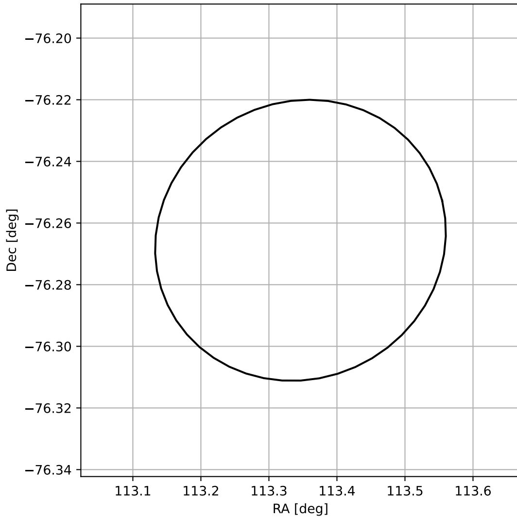
4FGL J0733.3-7615
