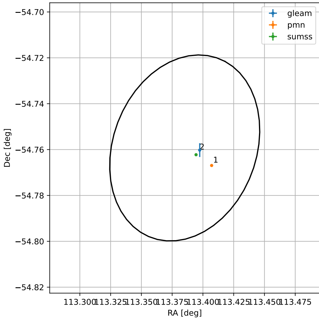
4FGL J0733.5-5445
