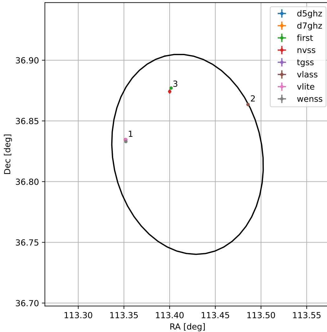
4FGL J0733.6+3649
