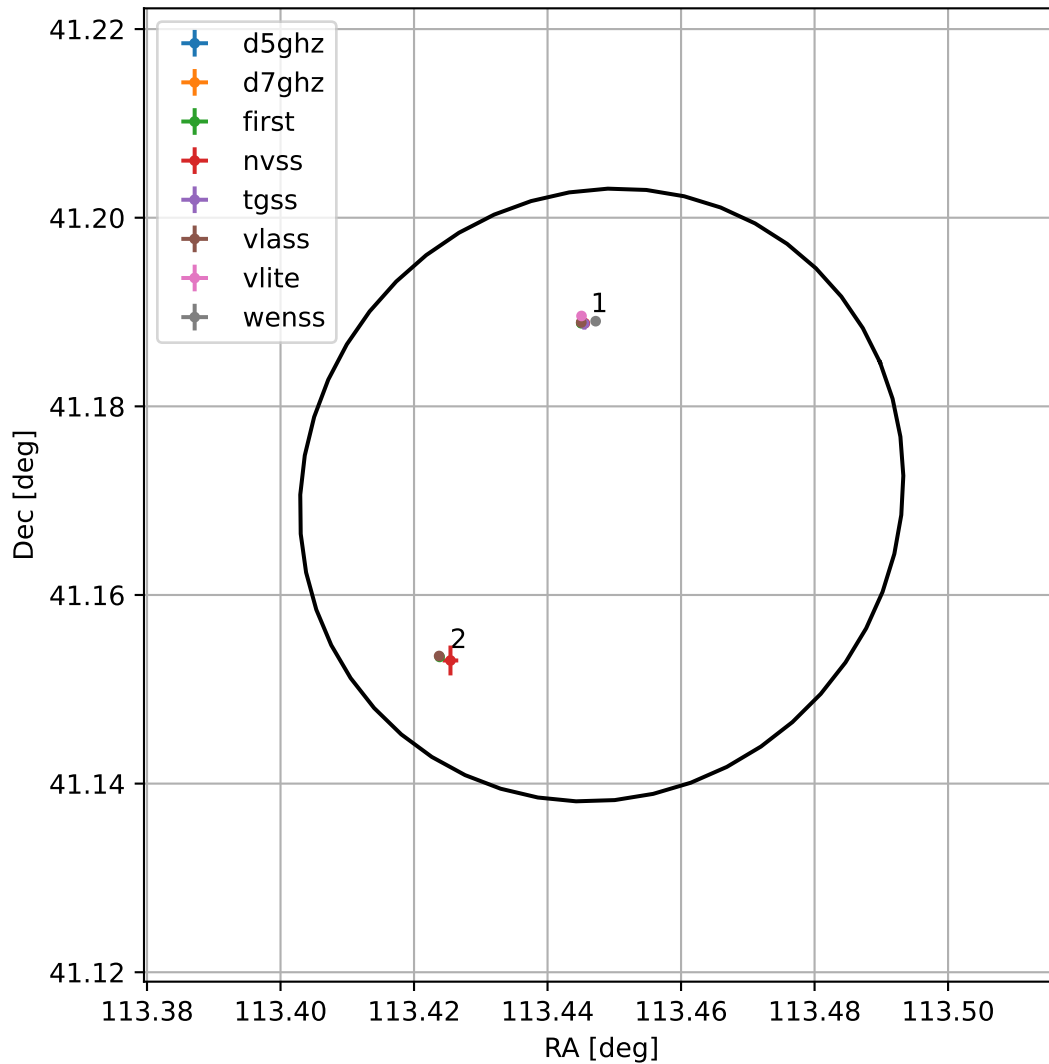
4FGL J0733.7+4110
